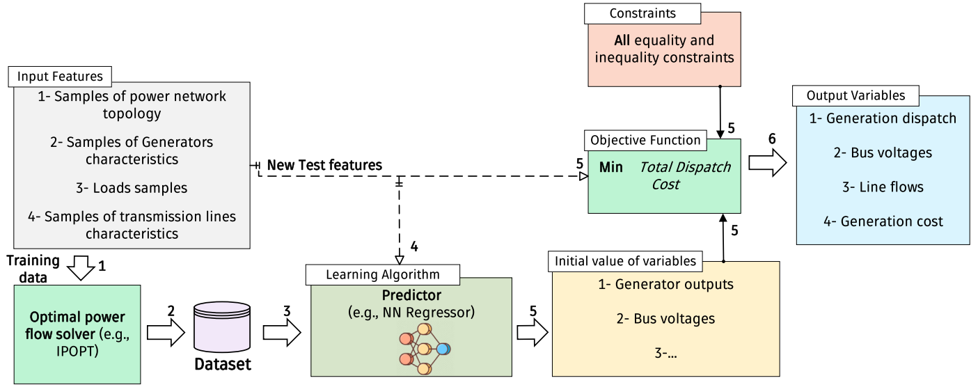
Fig. 4. Basic workflow diagram of the warm-start using learning algorithms.
