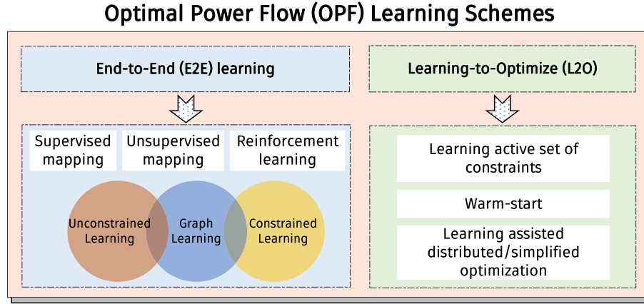
Fig. 1. Overview of OPF learning schemes.
