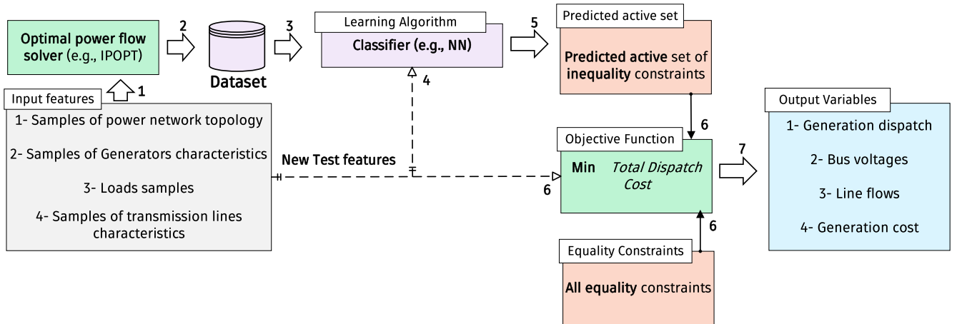
Fig. 3. Basic workflow diagram of learning active set of constraints.
