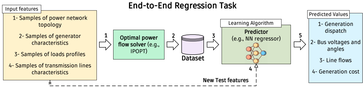
Fig. 2. Basic workflow diagram of the E2E OPF learning as a regression task.
